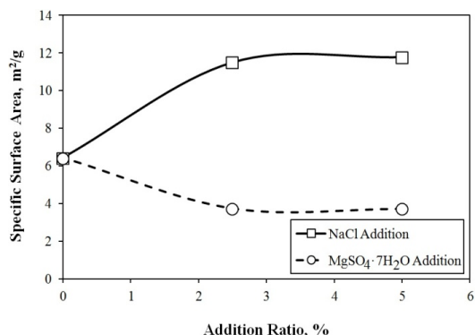
Figure 1. Variation of specific surface area with % addition
